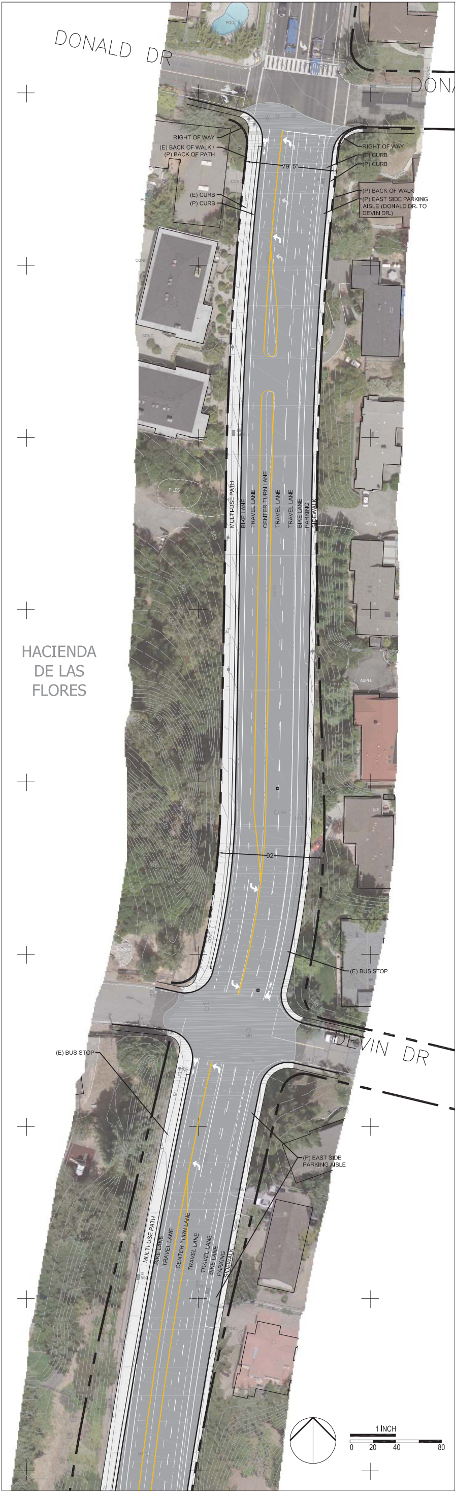
Livable Moraga Road Segment 3: Long-Term Option B
