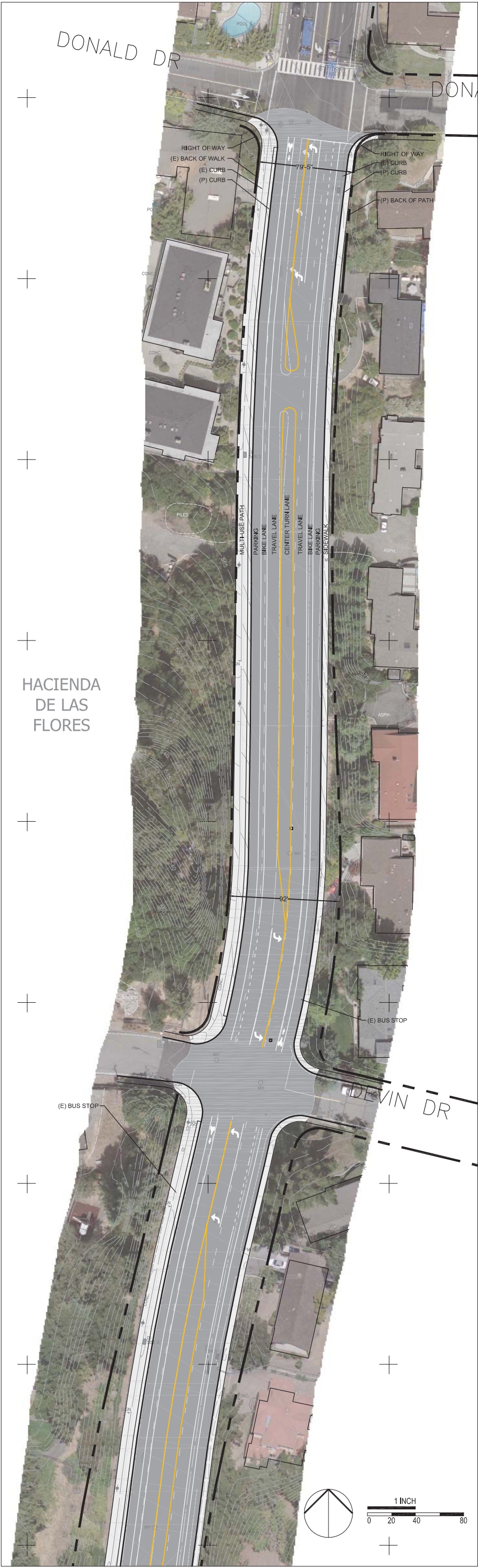
Livable Moraga Road Segment 3: Long-Term Option C
