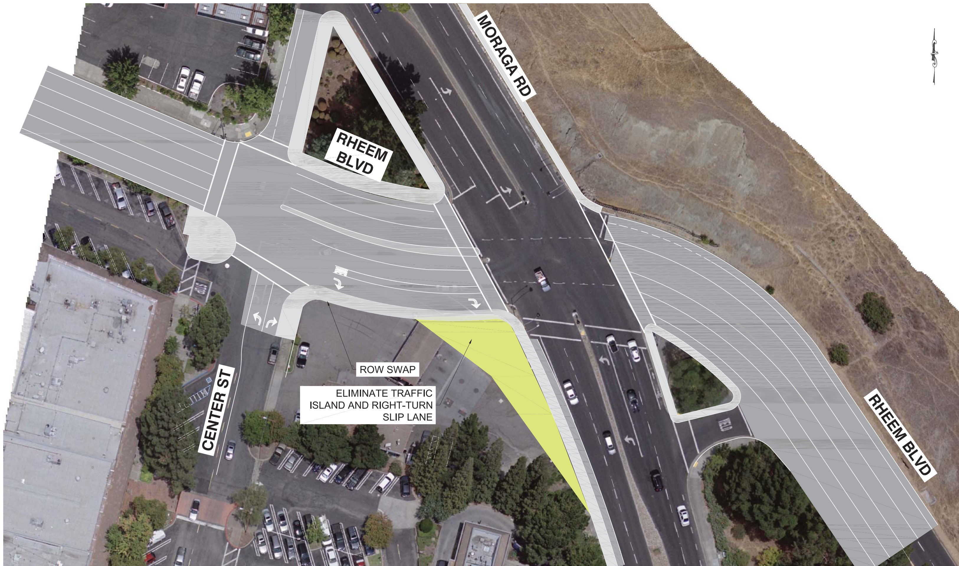
Moraga Rd/Rheem Blvd Intersection: Option 2
