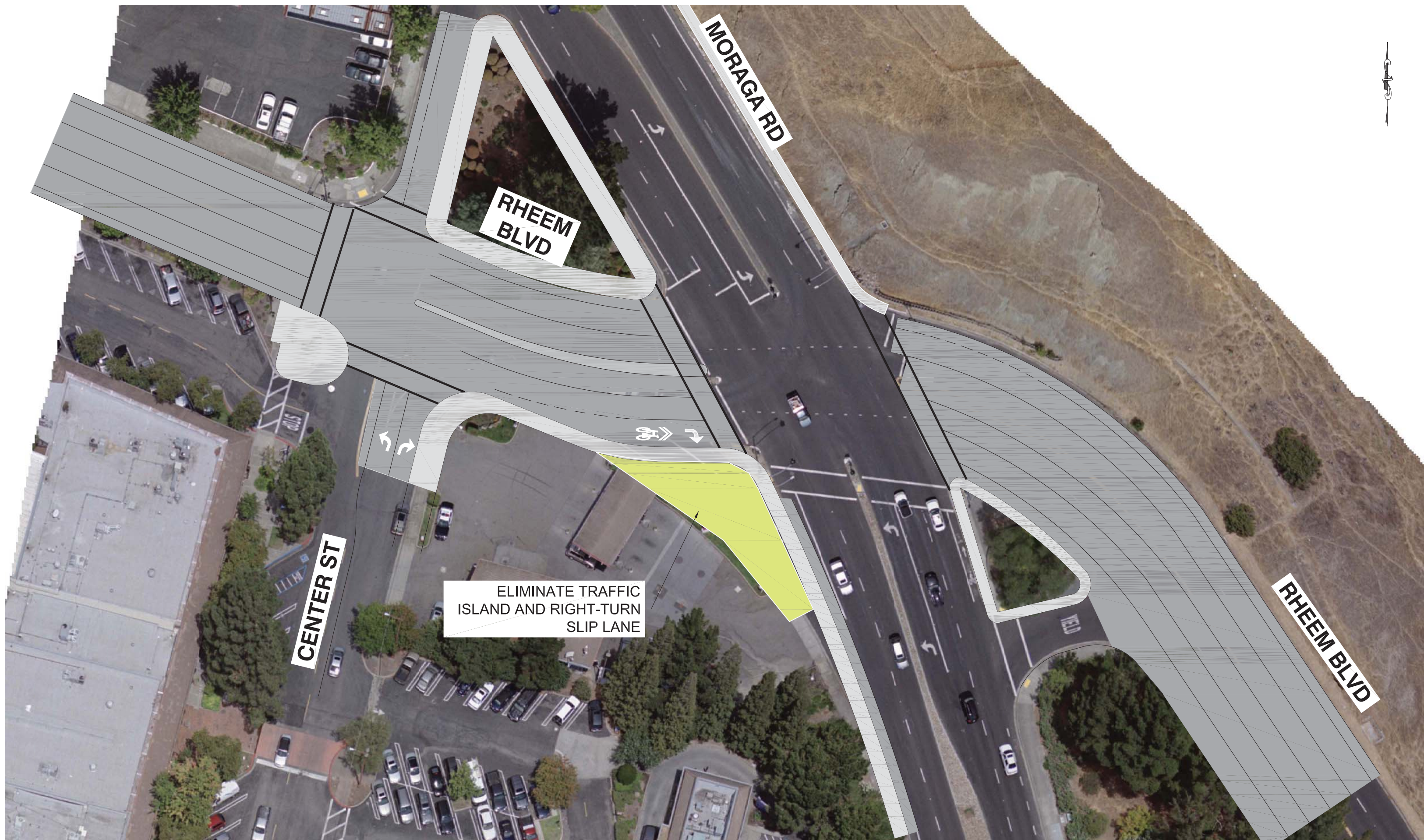
Moraga Rd/Rheem Blvd Intersection: Option 1
