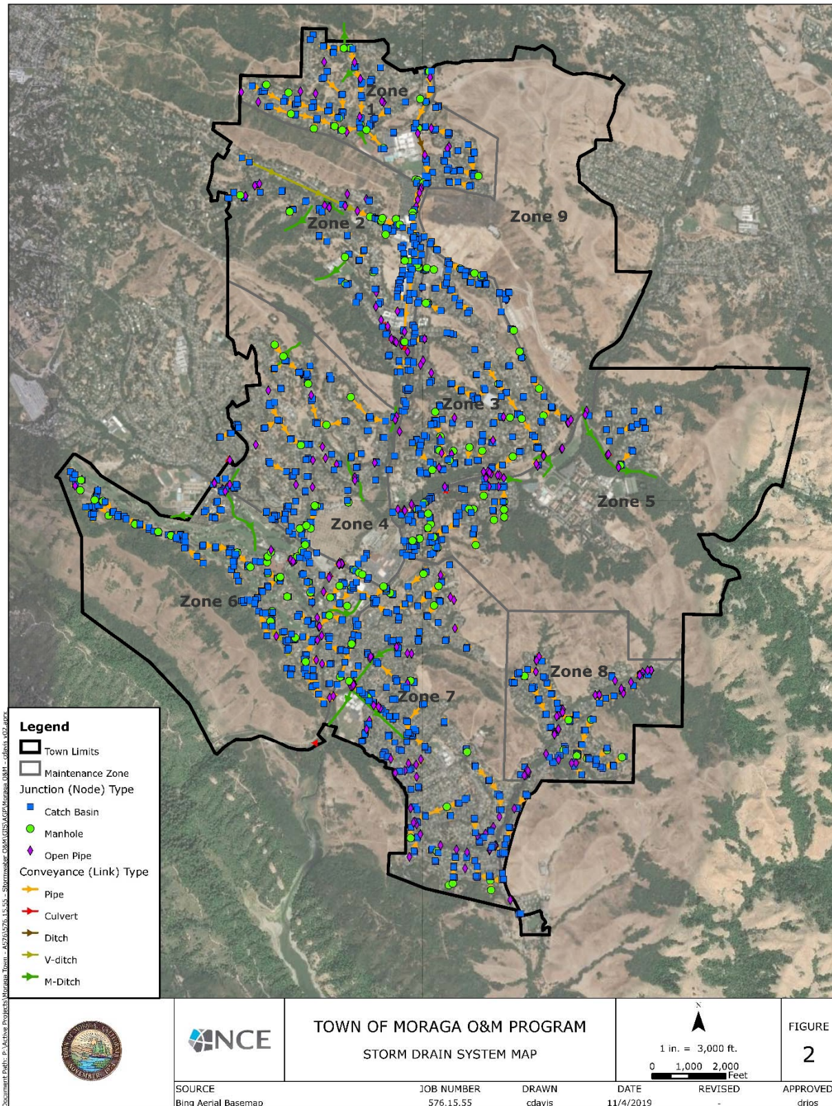
Figure 2: Storm Drain System Map
