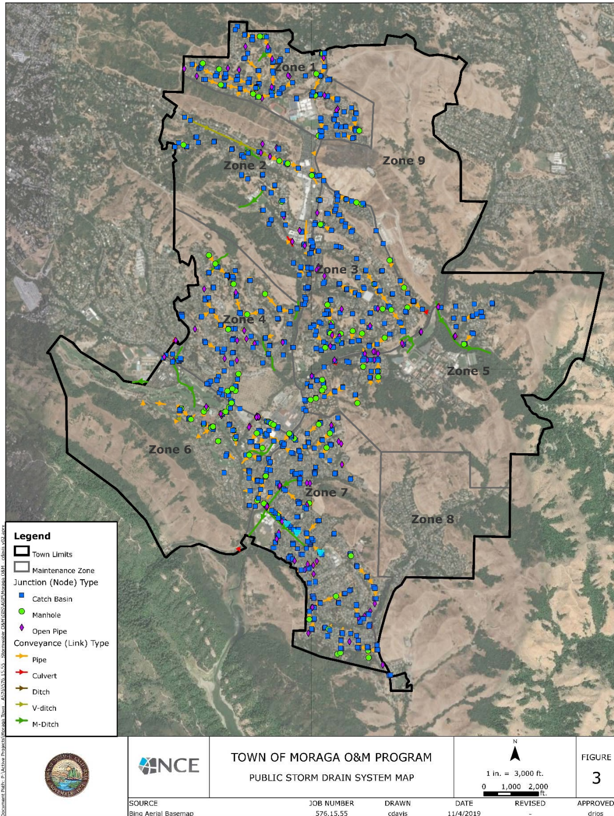
Figure 3: Public Storm Drain System Map
