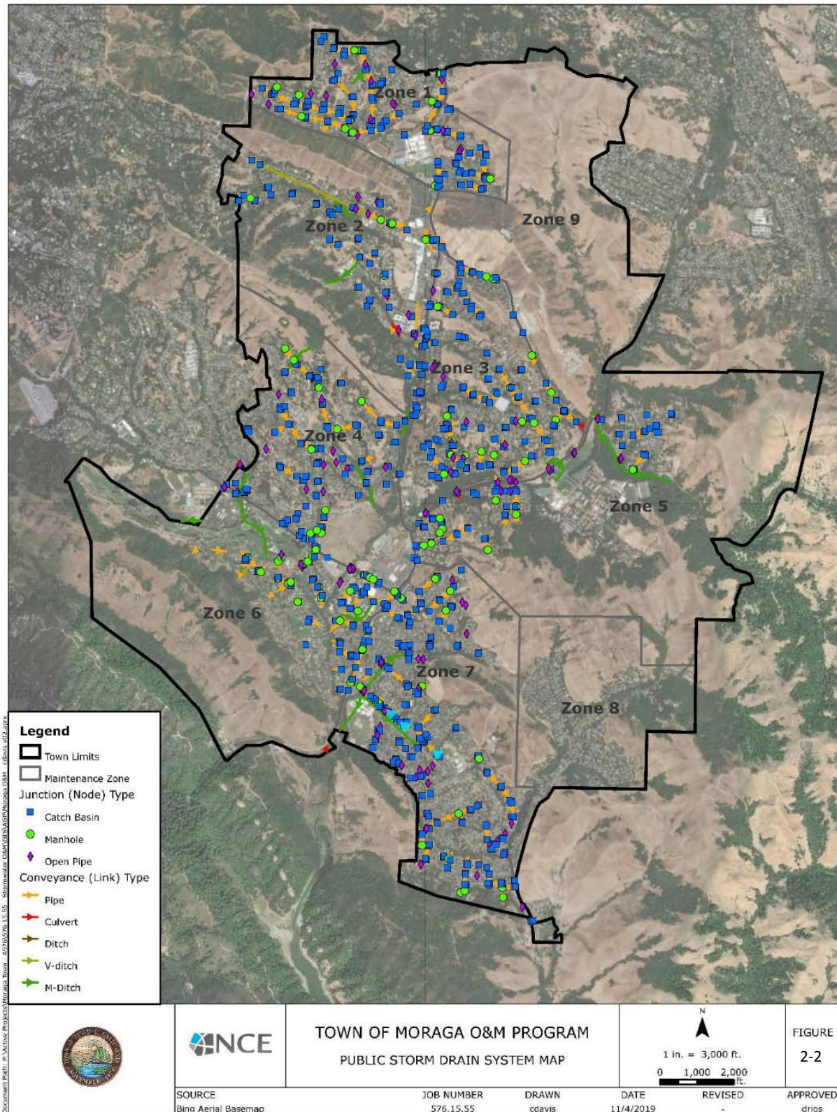
Figure 2-2. Public Storm Drain Infrastructure
